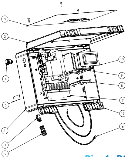
Diag 1 - DCCU
