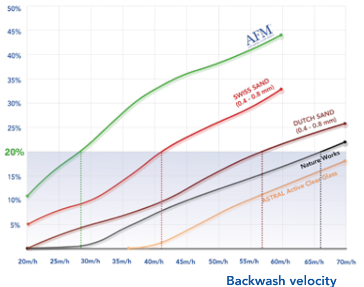
Filter bed expansion at 25°C
